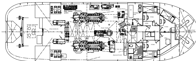
Below Maindeck
